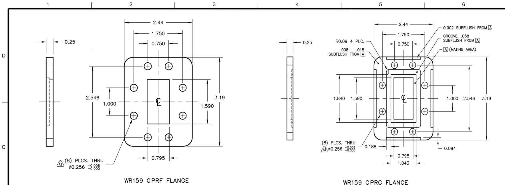
WR159 CPRG FLANGE
