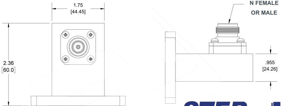
WR159 CPRG FLANGE
