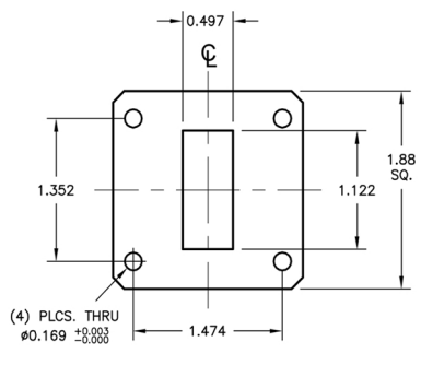
COVER FLANGE (F)
