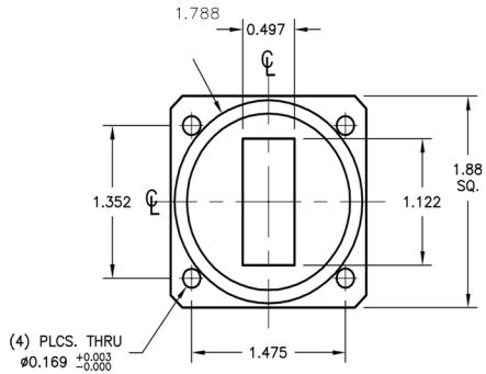
GROOVED FLANGE (O)
