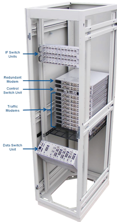
CRS-500 1:N Modem Redundancy System Typical Rack View (back side)
